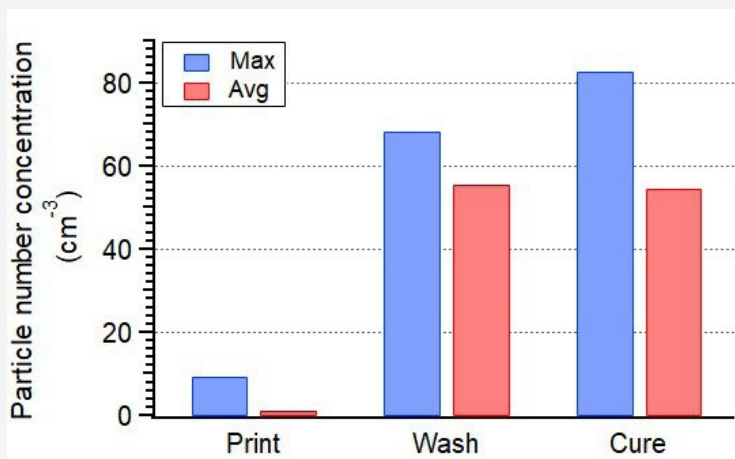
Figure 1: Maximum (Max) and average (Avg) total particle number concentrations for print, wash and cure processes.
