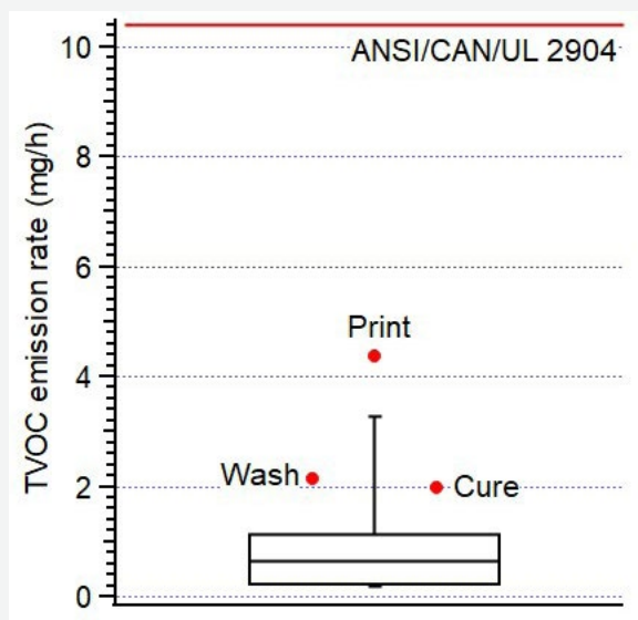
Figure 2: TVOC emission rates from this study (markers), compared to existing database (boxplot) and the maximum allowable level in ANSI/CAN/UL 2904 (red line). The box indicates 25% quartile, median and 75% quartile; the whiskers indicate the minimum and maximum values.
