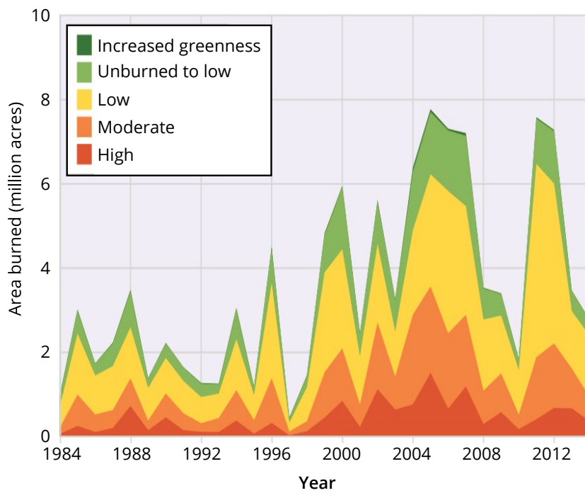
Figure 3: Damage caused by wildfires in the U.S. (1984-2014) obtained from U.S. EPA 9
